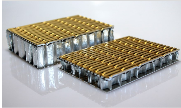
Picture 1-2: Two versions of the highly effective acoustic Composite (CMP) mesh with 12 and 25 mm thick honeycomb supporting plate and gold anodised Alu 6010 mesh.
