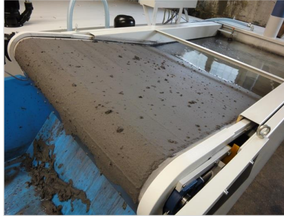
Picture 2: The self-cleaning MAXFLOW stainless steel belt.
